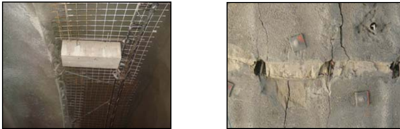
Picture 9: foam mortar blocks or special concrete composition
