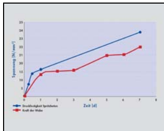
Picture 14: compressive strength
