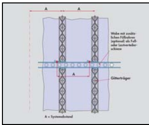
Picture 18: Honeycomb used as yieldable load transformation beam
